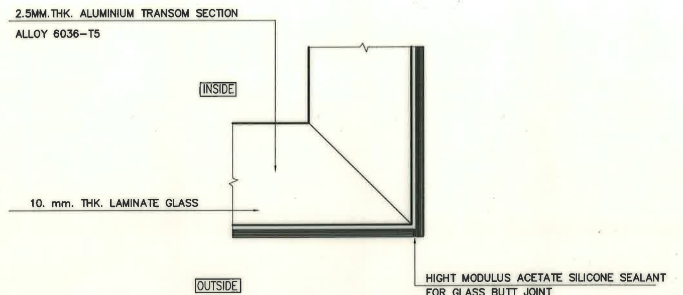
HORIZONTAL DETAIL
