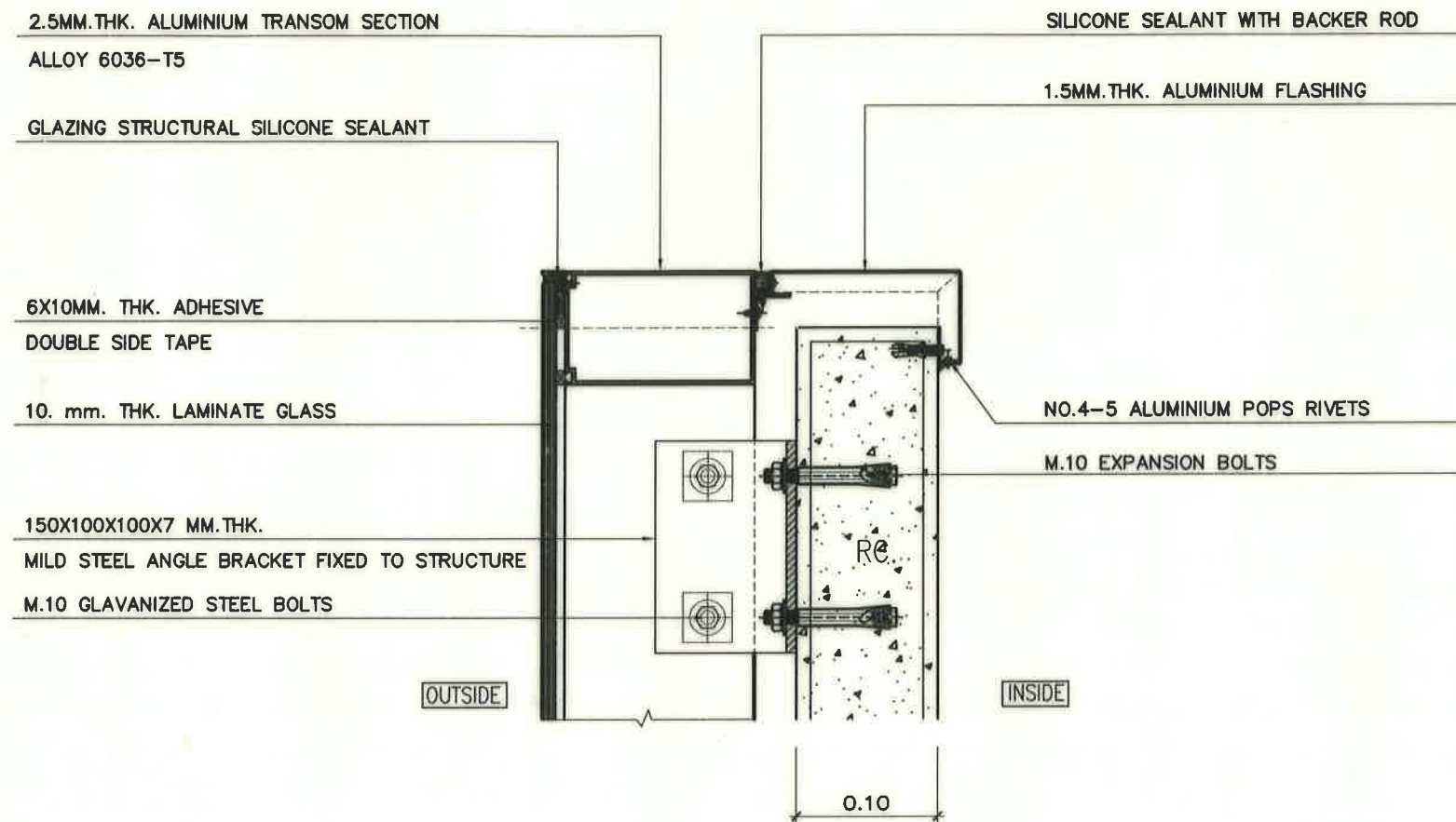
VERTICAL DETAIL
