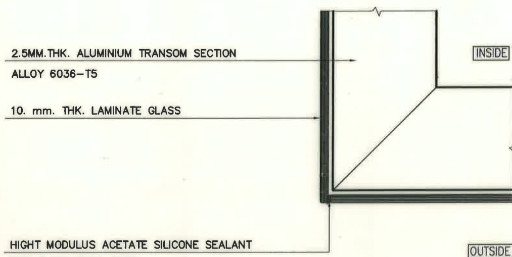
HORIZONTAL DETAIL
